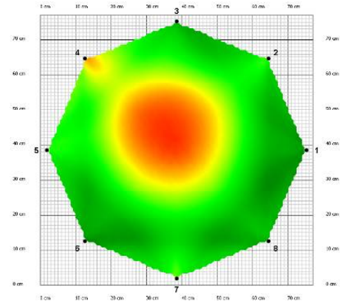
c) Tomogram of moderately infected oil palm sample 2
