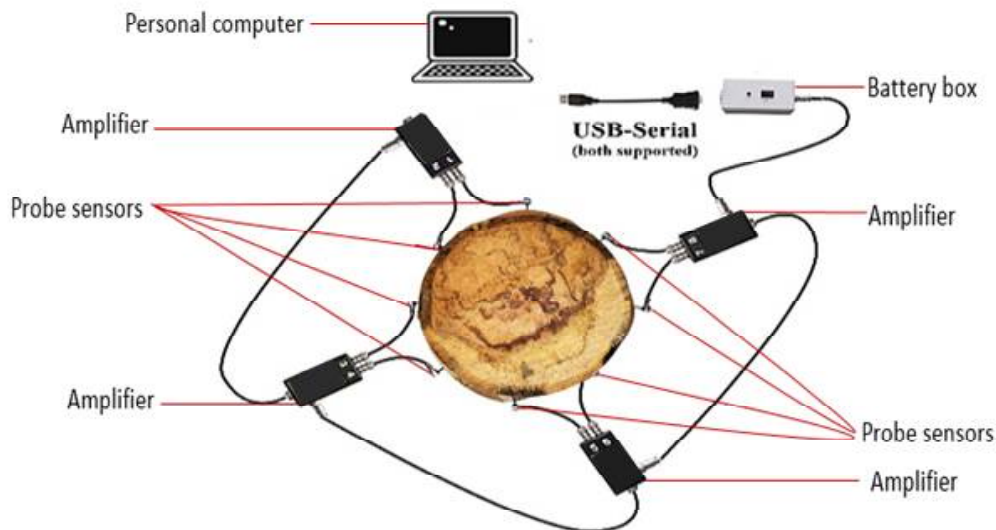
Figure 2 Experimental set-up of TomoSawit for acoustic tomography data acquisition
